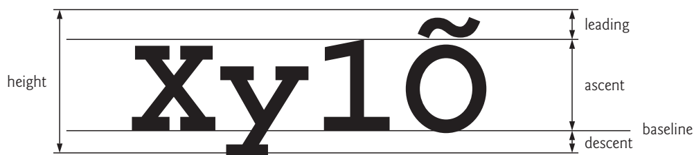
Fig. 15.13 | Font metrics.
