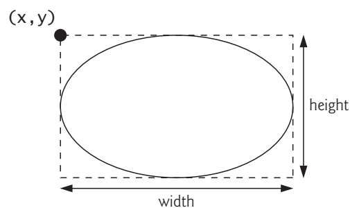
Fig. 15.21 | Oval bounded by a rectangle.
