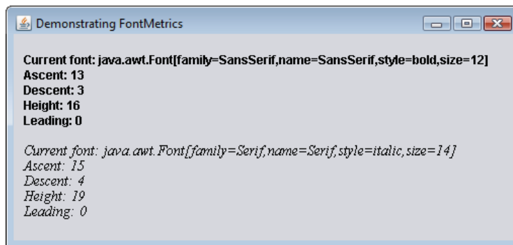
Fig. 15.16 | Creating JFrame to display font metric information.
