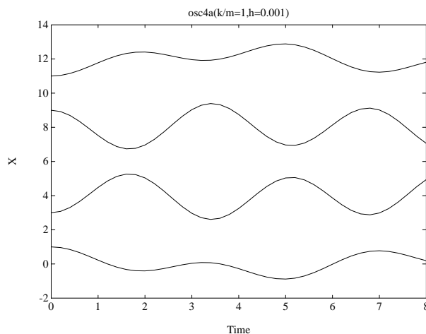
Figure 6: Illustration of the motion of a 4-particle system. The curves show the position of the 4 particles as functions of time. These results were for a system with k/m = 1 , k is the force constant, and m is the mass of a particle. The equilibrium positions of the particles are 0, 4, 8, 12. The parameter h is the time step used in integrating the equations of motion.
