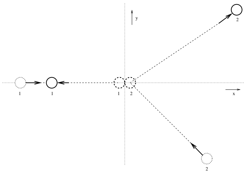
Figure 20: Collision of hard spheres in two dimensions: positions at one time unit before collision (dotted circles); at collision (dashed circle); and one time unit after collision (solid circles) are shown. Particles 1 and 2 are travelling at the same speed, s , before the collision. Particle 2 is travelling along a line that is 45^\circ from the x-axis. At collision they exchange x-components of velocity; their y-components of velocity are unchanged. Therefore, after collision particle 1 is travelling in the x-direction at speed s/\sqrt{2} , while particle 2 is travelling upward and to the right, at an angle of \arctan(1/\sqrt{2}) to the x-axis, with a speed equal to s\sqrt{3/2} .
