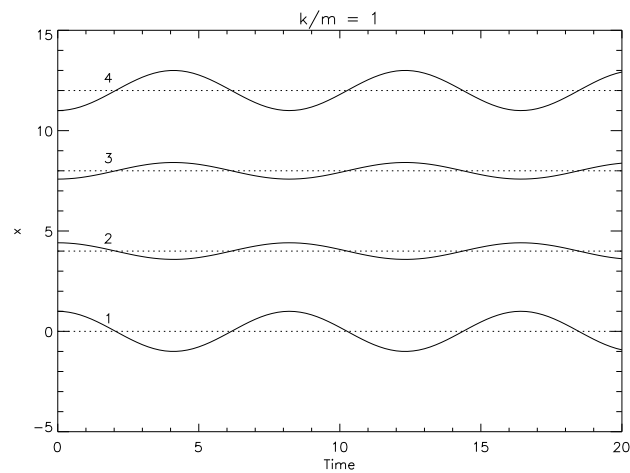
Figure 26: Illustration of the low-frequency mode of a four-particle system with k/m = 1 , \delta = 0 . Equilibrium positions of the four particles are assumed to be 0, 4, 8, 12.
