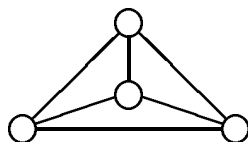
Figure 8: Minimum energy configuration for 4 particles in a 3-dimensional LJ model: particles are located at the corners of a regular tetrahedron.
