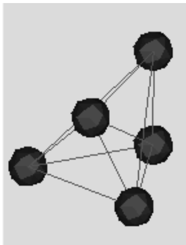
Figure 9: Minimum energy configuration for 5 particles.
