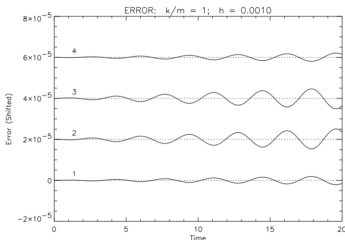
Figure 17: Error in numerical solution by Verlet's method of 1-dimensional, 4-particle HL model: h = 0.001 , k/m = 1 . The curves have been shifted vertically: the point of zero error for a particular curve is its position at t=0 .
