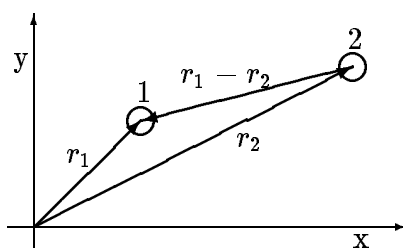
Figure 12: A 2-particle, 2-dimensional system.
