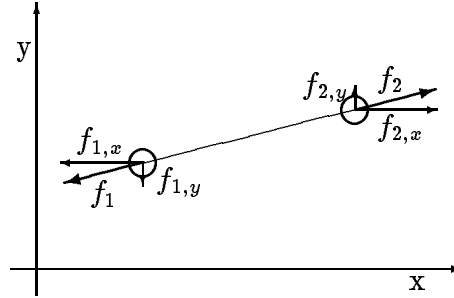
Figure 13: Force vectors in a 2-particle, 2-dimensional system.
