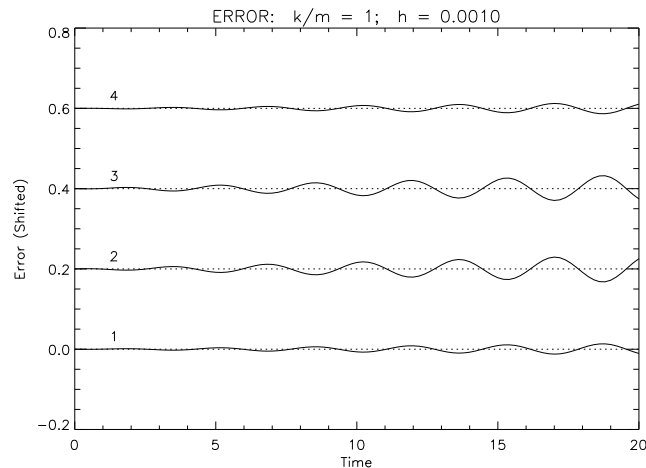
Figure 15: Error in numerical solution by Euler's method of 1-dimensional, 4-particle HL model: h = 0.001 , k/m = 1 . The curves have been shifted vertically: the point of zero error for a particular curve is its position at t=0 .
