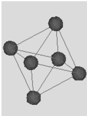
Figure 10: Minimum energy configuration for 6 particles.
