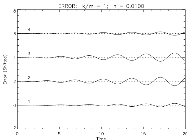
Figure 14: Error in numerical solution by Euler's method of 1-dimensional, 4-particle HL model: h = 0.01 , k/m = 1 . The curves have been shifted vertically: the point of zero error for a particular curve is its position at t=0 .
