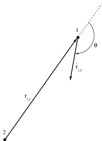
Figure 22: Illustration of necessary condition for a collision.
