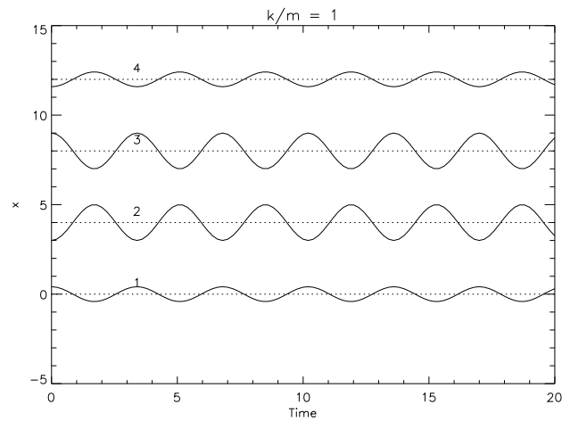
Figure 25: Illustration of the high-frequency mode of a four-particle system with k/m = 1 , \delta = 0 . Equilibrium positions of the four particles are assumed to be 0, 4, 8, 12.
