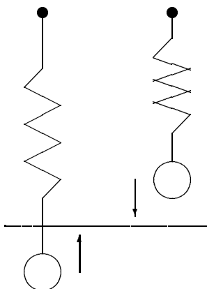
Figure 3: The motion of a small mass suspended from a spring typifies the motion of a particle subject to an HL force.
