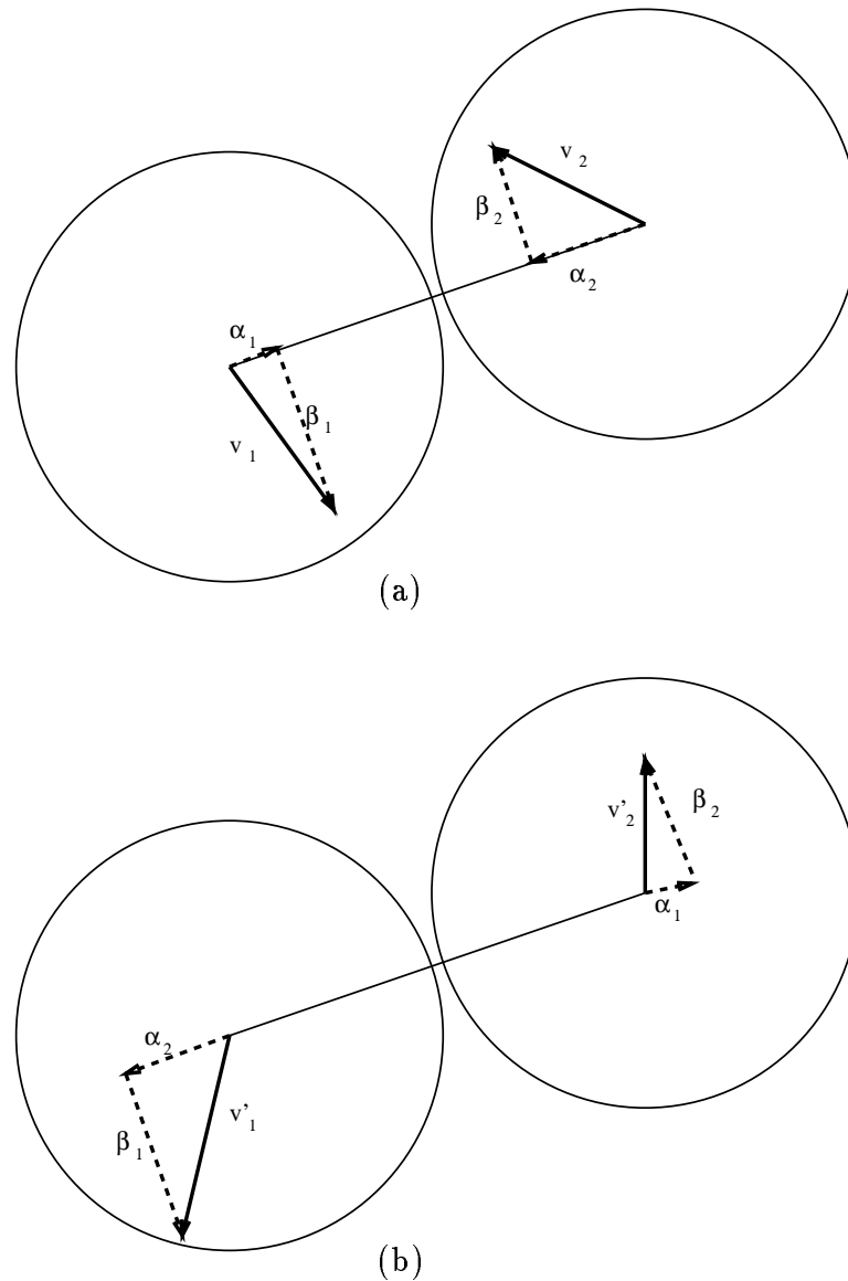
Figure 21: Detail of velocity components at instant before collision (a), and instant after collision (b). At collision the force is exerted only along the line joining the centers of the particles; no force is exerted in the plane perpendicular to this line because the particles are assumed to be smooth . Thus velocity components along this line are exchanged at the instant of collision, but velocity components in the plane perpendicular to this line are unchanged.
