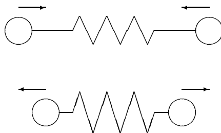
Figure 4: The motion of two small masses connected by a spring illustrates the nature of the motion of a 2-particle system in the HL model.
