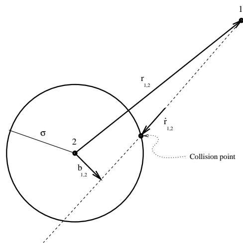
Figure 23: Illustration of collision parameters. Here r_{1,2} is the position of the center of particle 1 relative to the center of particle 2; and \dot{r}_{1,2} is the velocity of particle 1 relative to the velocity of particle 2. Thus you can think of particle 2 as fixed at the origin, and particle 1 at r_{1,2} moving with velocity \dot{r}_{1,2} . For a collision to occur particle 1 must be moving towards the origin, and must come within a distance \sigma (the particle's diameter) of the origin. Particle 1 is moving towards the origin if the dot product r_{1,2} \cdot \dot{r}_{1,2} < 0 as in this picture. In this picture \|b_{1,2}\| is the distance of closest approach by particle 1 to the origin: b_{1,2} is a vector perpendicular to \dot{r}_{1,2} . The point at which the collision occurs is the point where the trajectory of particle 1 crosses the circle of radius \sigma around the origin, and the time of collision is the time it takes to move from r_{1,2} to this point travelling at velocity \dot{r}_{1,2} .
