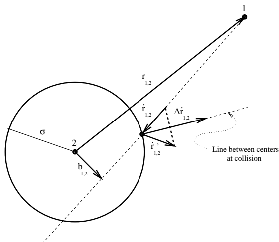
Figure 24: Change in velocity at collision of hard spheres. Parameters \sigma , r_{1,2} , r'_{1,2} , b_{1,2} are as defined in figure 22; r'_{1,2} is the relative velocity after collision and \Delta r'_{1,2} is the change in relative velocity due to the collision. Note that \Delta r'_{1,2} is perpendicular to the line between centers at the time of collision.
