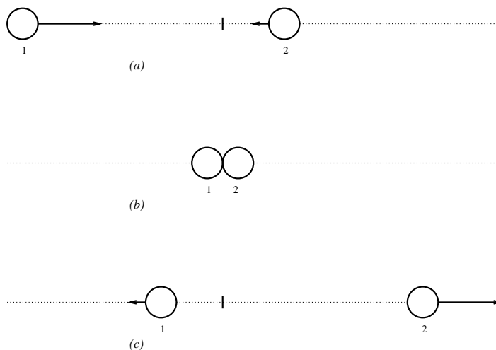
Figure 18: Collision of hard sphere particles in one dimension: (a) one time unit before collision; (b) instant of collision; (c) one time unit after collision. In this illustration particle 1 is travelling at four times the speed of particle 2 before the collision. At collision the particles exchange velocities so after the collision particle 2 is travelling at four times the speed of particle 1.
