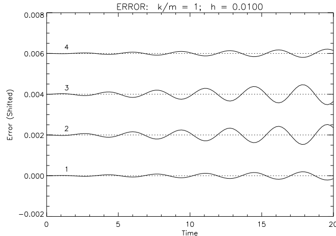
Figure 16: Error in numerical solution by Verlet's method of 1-dimensional, 4-particle HL model: h = 0.01 , k/m = 1 . The curves have been shifted vertically: the point of zero error for a particular curve is its position at t=0 .
