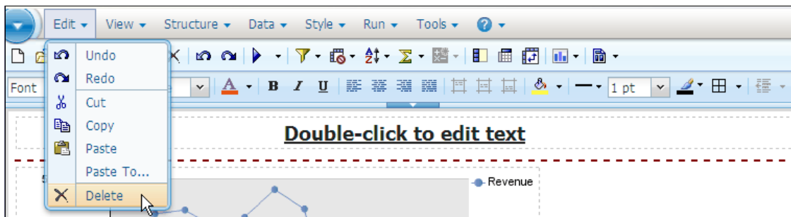
Figure 7-45 Deleting option
