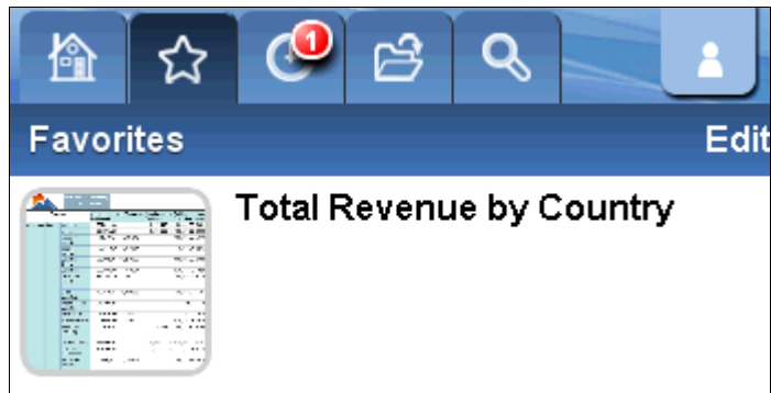
Figure 8-16 Favorites tab
