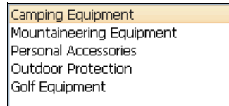
Figure 8-5 List box
