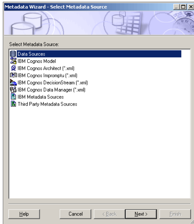
Figure 9-3 Metadata source
