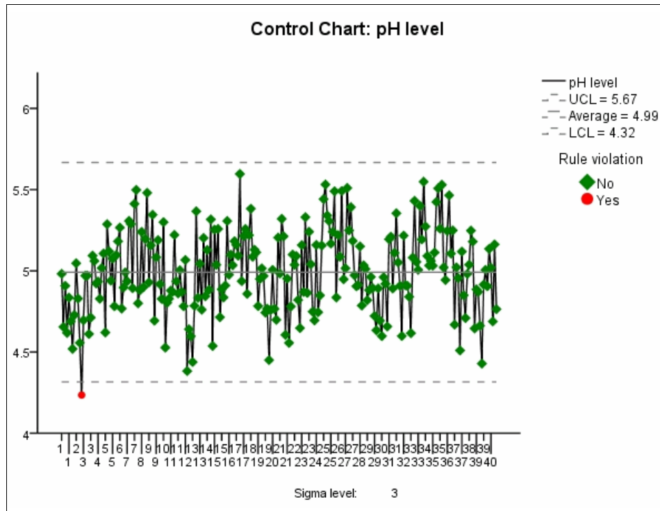
Figure 7-168 Individuals chart
