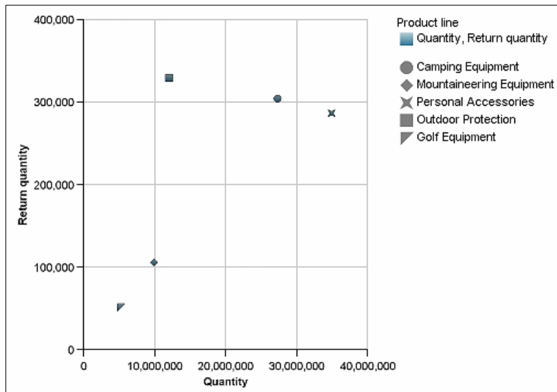
Figure 5-9 Scatter chart
