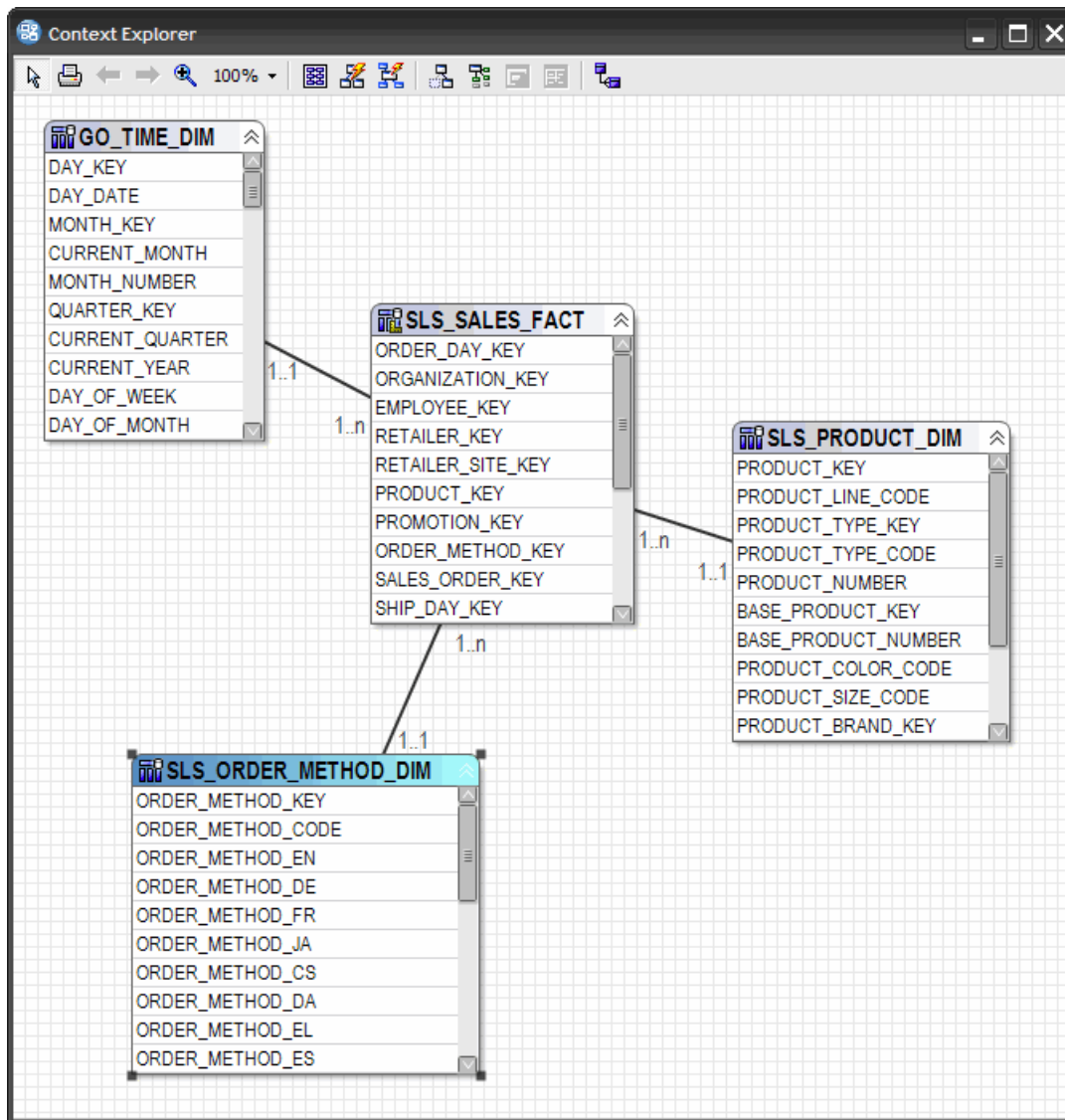
Figure 4-36 Context Explorer
