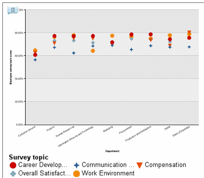
Figure 5-7 Point chart
