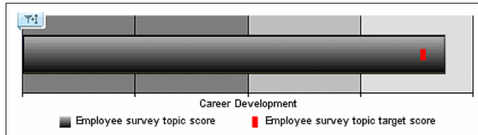
Figure 5-13 Bullet chart
