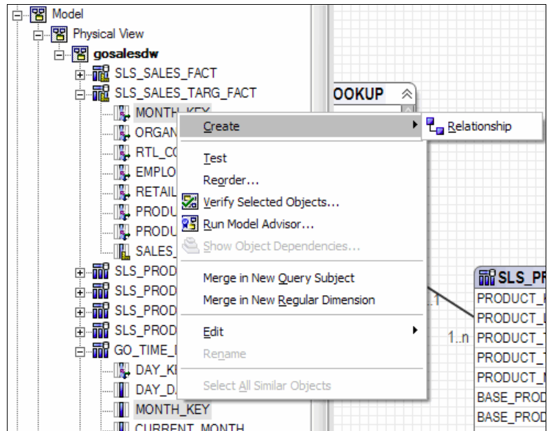
Figure 4-43 Create Relationship
