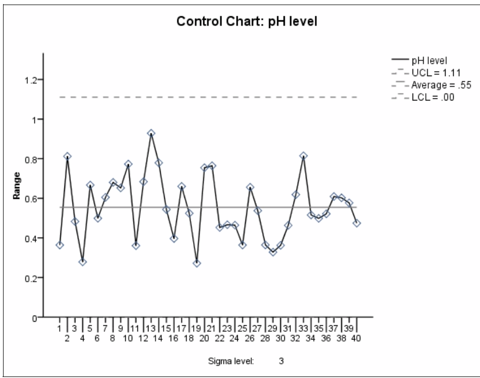
Figure 7-165 R chart
