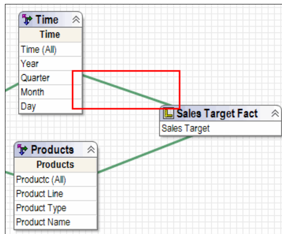
Figure 4-13 Scope relationship
