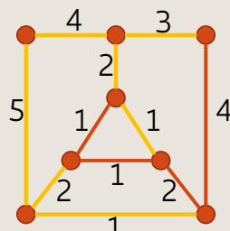
Dijkstra algorithm (SPT)
