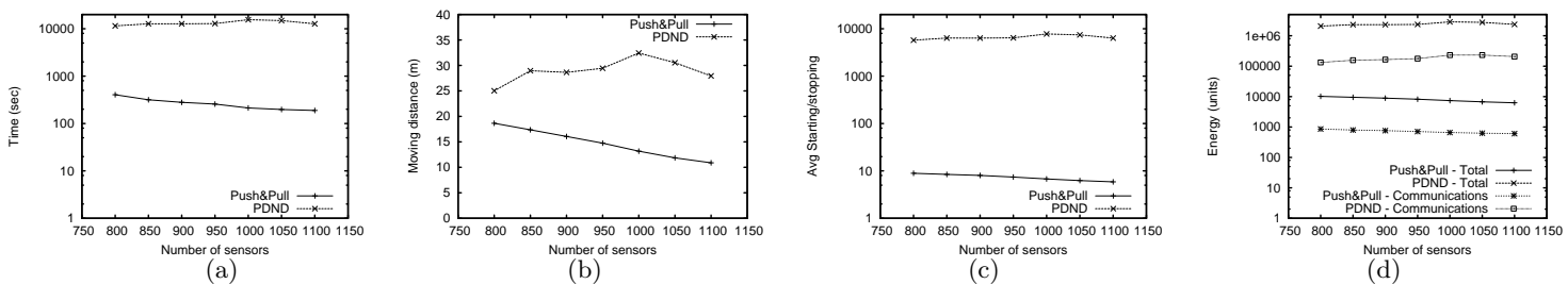
Figure 4: Performance comparisons between \delta -Push&Pull and PDND
