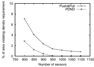
Figure 5: Percentage of area not meeting the density requirements.
