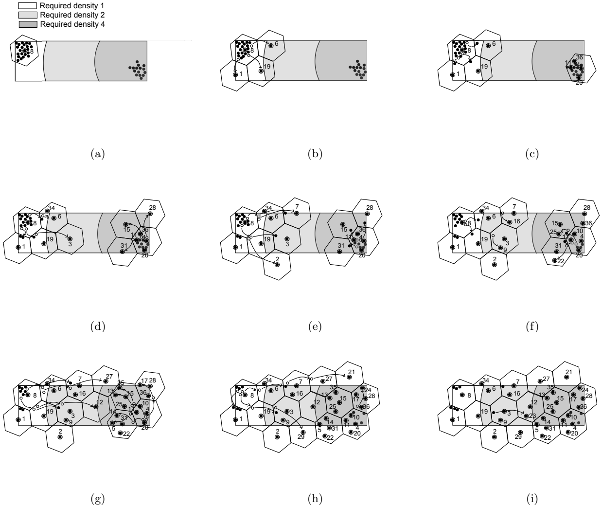
Figure 1: Algorithm execution: an example
