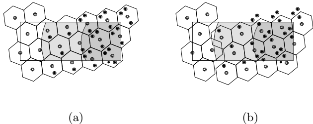
Figure 2: Coverage holes at the borders of the circular crowns during the execution of the alternate activation of the adjunct-snapped sensors.
