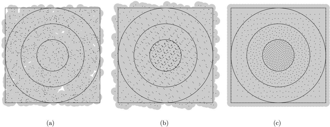
Figure 3: Initial configuration (a). Final deployment under \delta -Push&Pull (b) and PDND (c).
